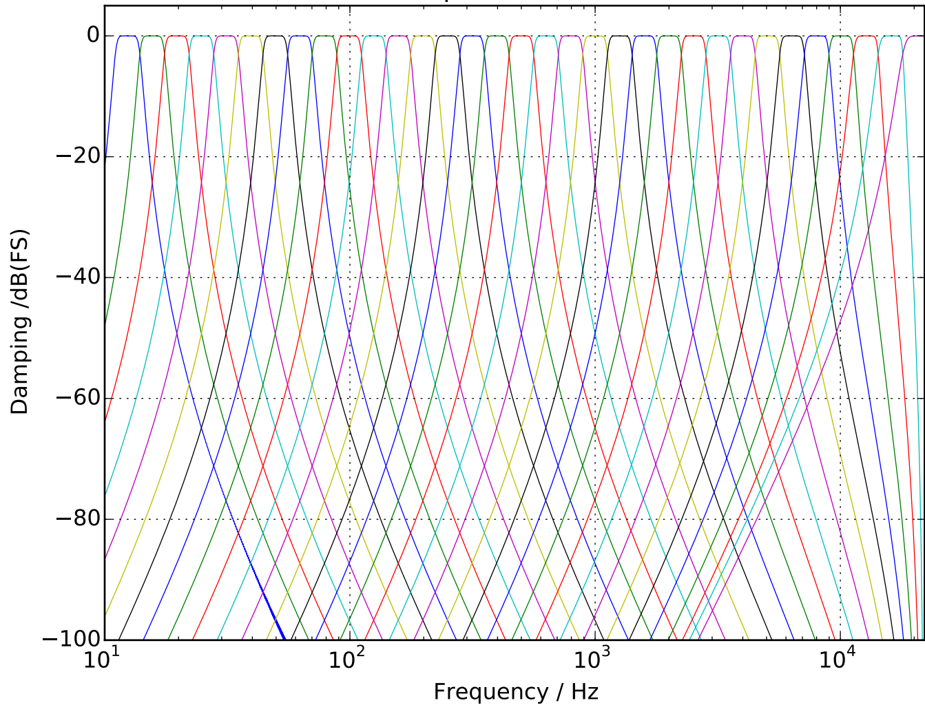
freqz() Filter Bank
